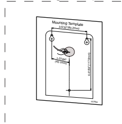
Mounting Template
